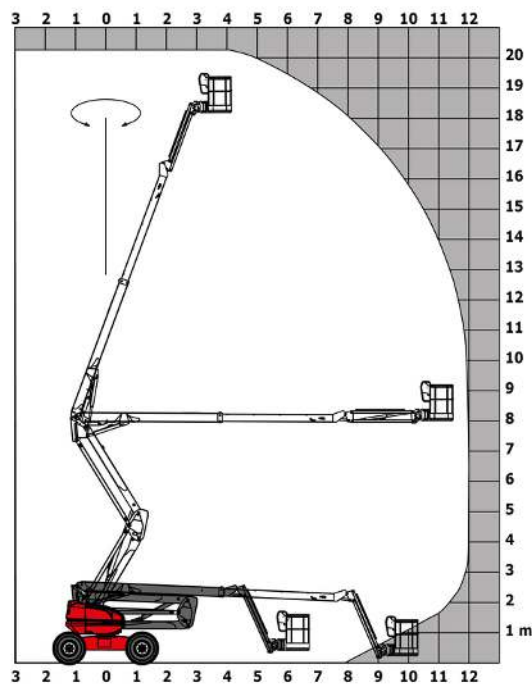
Laaddiagram
