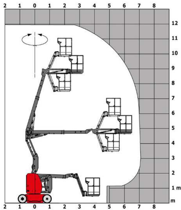
Laaddiagram
